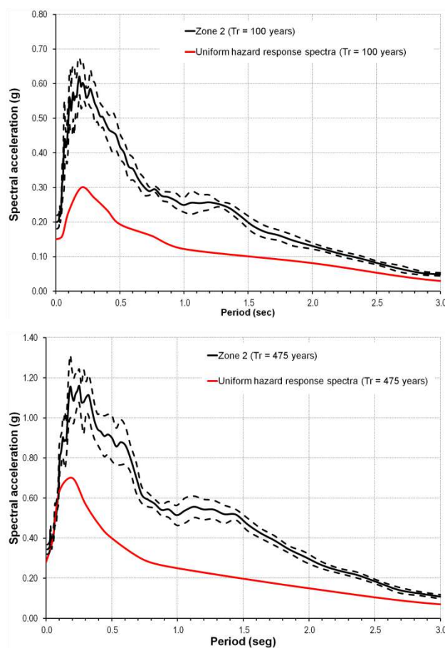
Figure 12: Response spectrums for Zone 2 of Case 2
