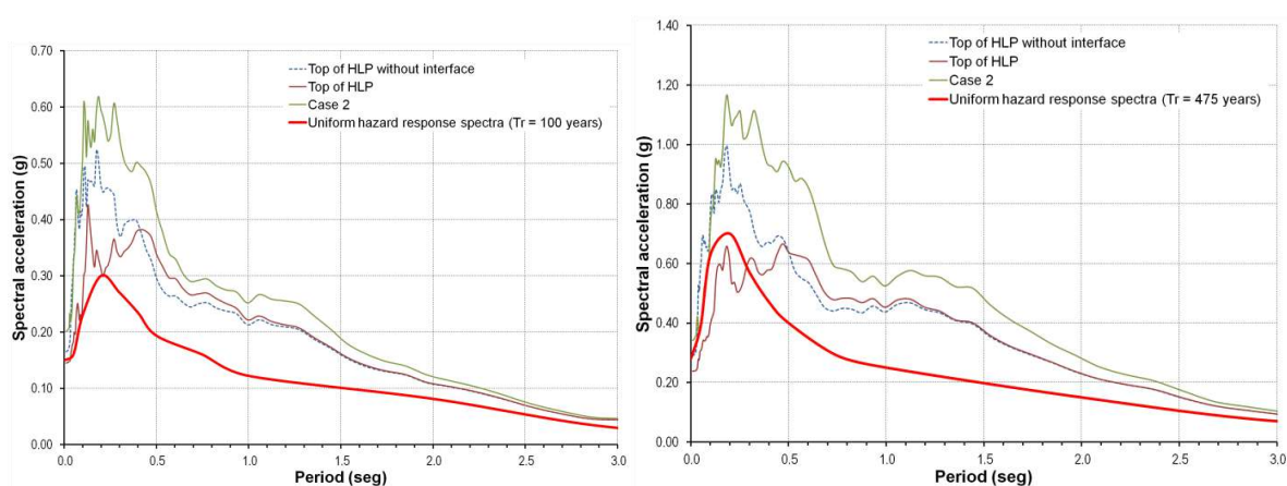
Figure 15: Response spectrums for column K for Case 3
