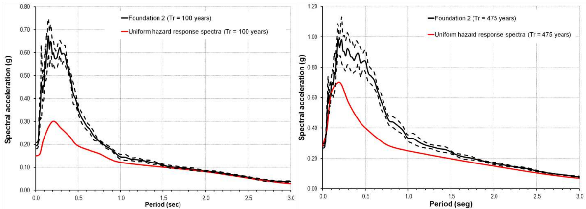
Figure 9: Response spectra for Foundation 2 type of Case 1
