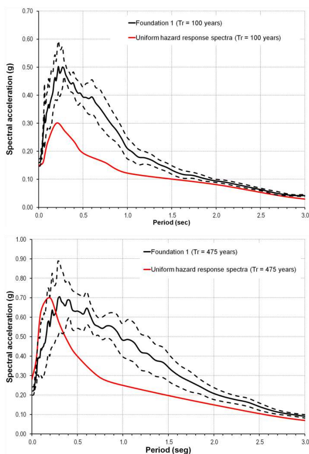
Figure 8: Response spectrums for Foundation 1 type of Case 1
