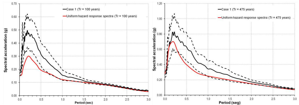
Figure 11: Average response spectra for Case 1
