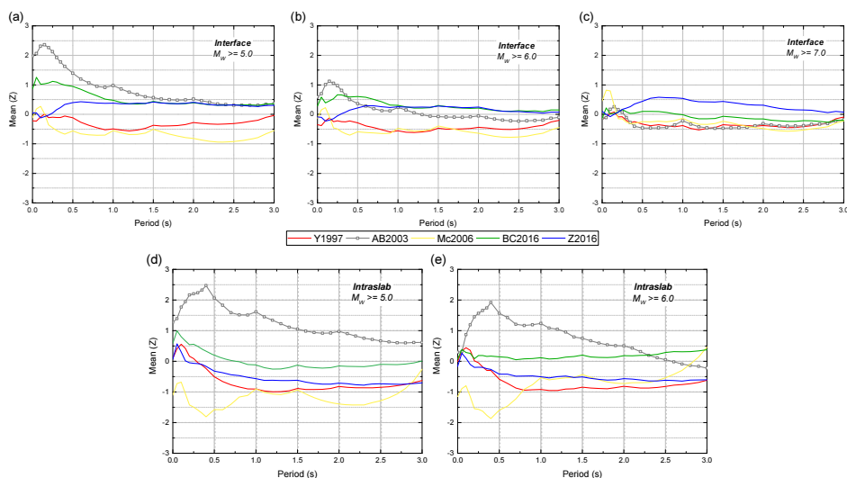
Figure 2. Mean of normalized residual distribution versus period response, according to moment magnitude and type of event. (a,b,c) interface events and (d,e) intraslab events.
