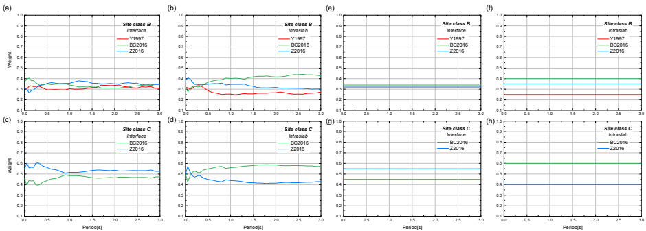
Figure 4. Weights assign to each GMPEs according to the type of the event and site class B and C. a,b,c,d). Weights computed according to LLH values. e,f,g,h) Homogenized weights for all response periods.
