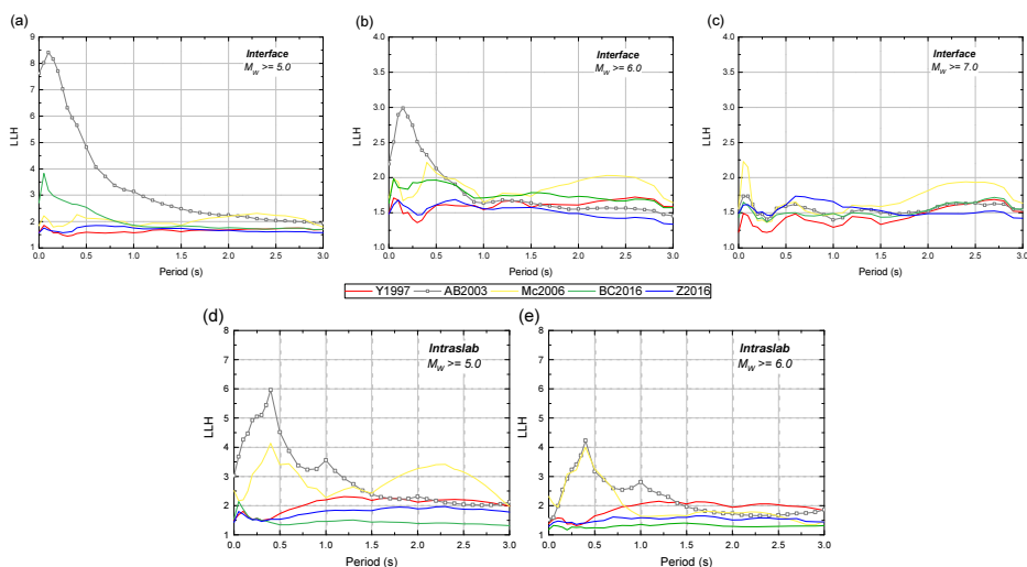
Figure 3. LLH values for different GMPEs assessed against observations, versus period response, according to magnitude and type of event. (a,b,c) interface events and (d,e) intraslab events.
