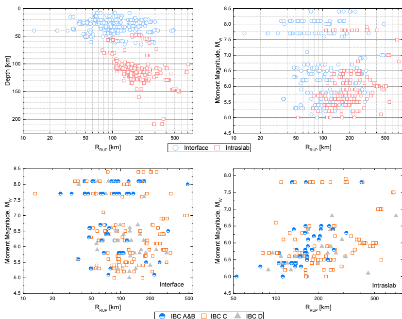
Figure 1. Dataset distribution regarding moment magnitude, focal depth, the closest distance to fault plane, and site class.
