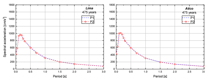
Figure 5. Uniform hazard spectrums for rock sites (site class B) and 475 years return period in Lima and Atico cities considering the weighting schemes “P1” and “P2”.
